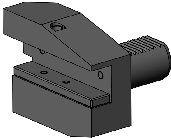
90 DEGREE VDI40 STATIC TOOL OUTPUT: 25mm SQR SHANK COOLANT: EXTERNAL
